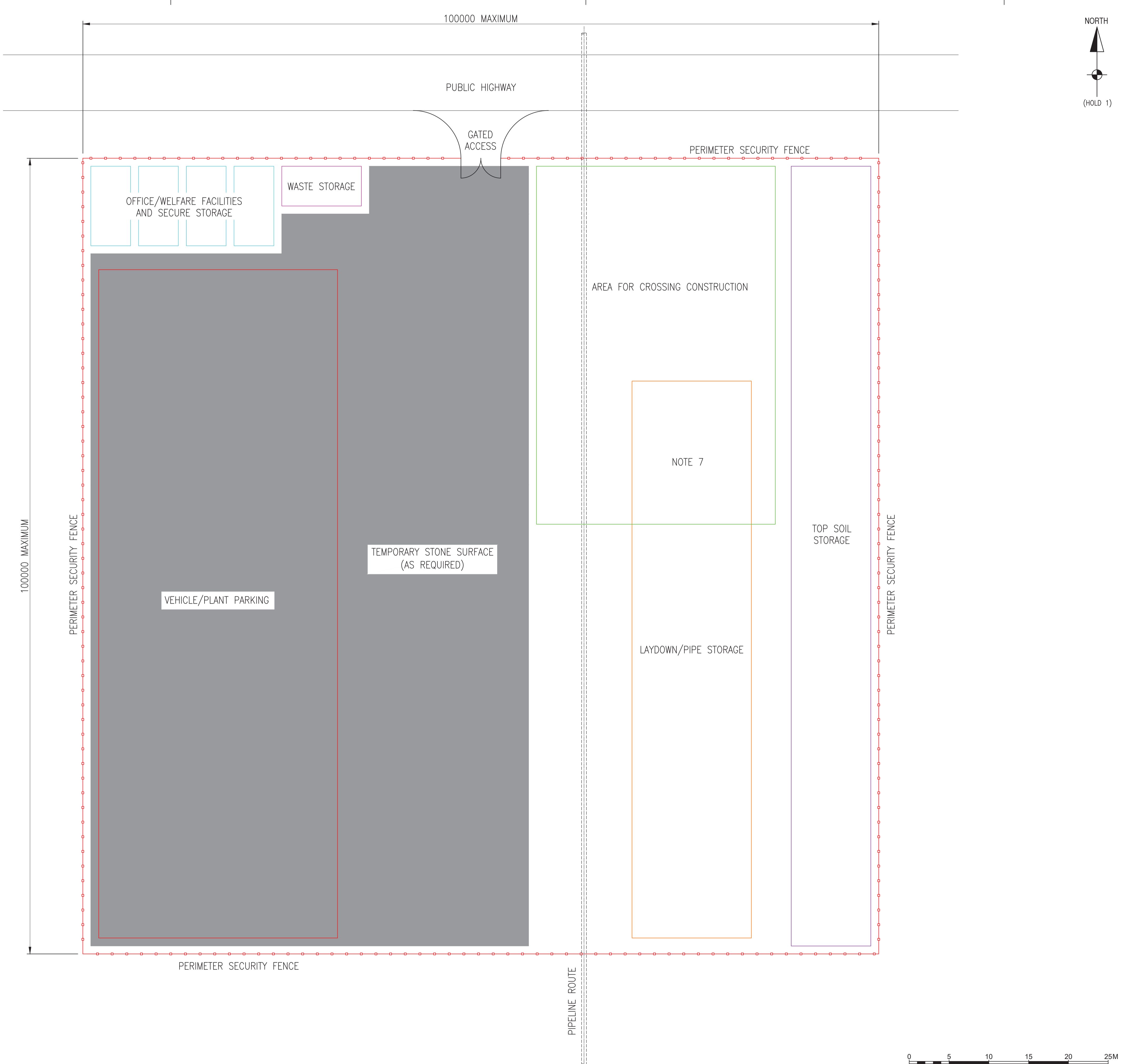
TYPICAL PLAN OF LAYDOWN, WELFARE AND PARKING AREA SCALE 1:250
